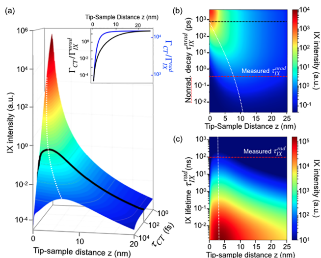
Figure 4. Simulations of IX PL dependence on \tau_{CT} , \tau_{IX}^{\text{nrad}} , and \tau_{IX}^{\text{rad}} . (a) Simulation of IX emission intensity for \tau_{CT} ranging from 1 fs to 10 ps with measured data overlaid in black. (inset) Fitted values for distance-dependent rate parameters. (b) Simulation of IX emission intensity for \tau_{IX}^{\text{nrad}} from 1 fs to 7 ns with measured \tau_{IX}^{\text{nrad}} = 0.6 ps (red, dashed line). (c) Simulation of IX emission intensity for \tau_{IX}^{\text{rad}} from 1.5 ps up to 1500 ns with measured \tau_{IX}^{\text{rad}} = 94 ns (red, dashed line). Peak intensity evolutions (white, dashed lines) are shown for all simulations.
