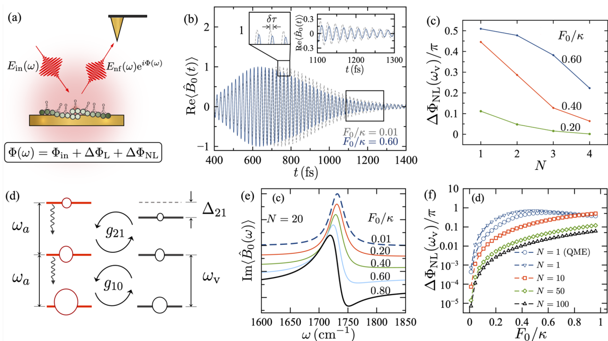
FIG. 5. Power-dependent phase rotation of the vibrational coherence. (a) Schematic picture of coherently scattered fields in molecule-coupled resonators. The output phase contains the driving phase \Phi_{\text{in}} as well as linear and nonlinear phase shifts, \Delta\Phi_{\text{L}} and \Delta\Phi_{\text{NL}} . (b) Evolution of the collective coherence \text{Re}\langle\hat{B}_0(t)\rangle for N = 3 anharmonic vibrations ( U = 20 \text{ cm}^{-1} ) subject to a single 155 fs pulse centered at 600 fs with driving strength parameters F_0/\kappa = 0.6 (solid line) and F_0/\kappa = 0.01 (dashed line). The delay \delta\tau between the weak and strong field responses is highlighted. The inset shows a magnified view of the FID signal after the pulse is over (boxed region). (c) Nonlinear phase \Delta\Phi_{\text{NL}} at bare resonance ( \omega_{\text{v}} = 1732 \text{ cm}^{-1} ) as a function of the molecule number N , obtained from exact solutions of the quantum master equation. Curves are shown for different values of F_0/\kappa . (d) Level scheme for resonant coupling between the antenna photon levels with anharmonic vibrations in the presence of a strong pulse. The ground and first excited levels exchange coherence and population resonantly, but the transition from the first to the second vibrational level is detuned from the antenna by \Delta_{21} = 2U . Level populations at the pulse maximum are represented as circles of different sizes. g_{10} and g_{21} denote state-dependent Rabi frequencies. (e) Imaginary part of the FID signal in the frequency domain for anharmonic oscillators with \Delta_{21} = 40 \text{ cm}^{-1} , obtained from the nonlinear chirping model. Curves are labeled by the ratio F_0/\kappa . (f) Nonlinear phase \Delta\Phi(\omega_{\text{v}}) as a function of the ratio F_0/\kappa , as predicted by the nonlinear chirping model. Curves are shown for different molecule numbers N . Exact results from the quantum master equation for N = 1 are also shown for comparison. We set \omega_{\text{v}} = \omega_{\text{a}} = \omega_{\text{d}} with other parameters as in Fig. 2.
