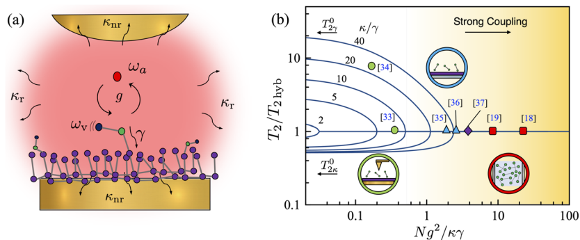
FIG. 1. Infrared nanocavity quantum electrodynamics. (a) A nanocavity confined infrared photon field resonant at frequency \omega_a with radiative decay rate \kappa_r and non-radiative decay \kappa_{nr} coupled with a molecular vibration with absorption frequency \omega_v and vibrational relaxation rate \gamma . The total photon decay rate is \kappa = \kappa_r + \kappa_{nr} . The cavity photon exchanges energy with the material quantum states at rate g . (b) Photonic ( T_{2\kappa} ) and material ( T_{2\gamma} ) dephasing times as a function of the cooperativity parameter Ng^2/\kappa\gamma . For small cooperativities (weak coupling), the photonic and material dephasing times are different when \kappa \neq \gamma . For cooperativities that exceed unity (strong coupling), a single hybrid dephasing time T_{2\text{hyb}} is established. Selected infrared cavity implementations using tip-enhanced IR antenna resonators 33,34 (green circles), planar nanocavities 35,36 (blue triangles), intersubband quantum well heterostructures 37 (purple diamond), and liquid-phase Fabry–Perot microcavities 18,19 (red squares) are given.
